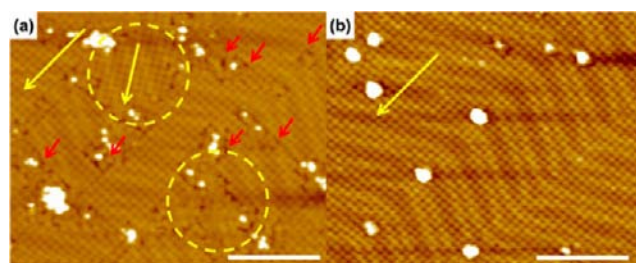
Figure 7. Empty-state STM images of a CuPc monolayer dosed with a supersonic MBS (molecular beam source). Scale bars are 20 nm. (a) CuPc monolayer dosed with ozone (O 3 ) for 10 min at 25 °C ( V_s = 2.0 V, I_t = 20 pA, fMBS = 30 Hz). Red arrows indicate subsurface crack sites. (b) CuPc monolayer dosed with NO for 10 min at 25 °C ( V_s = 2.0 V, I_t = 20 pA, fMBS = 30 Hz). Yellow arrows indicate the orientation of CuPc domains.
