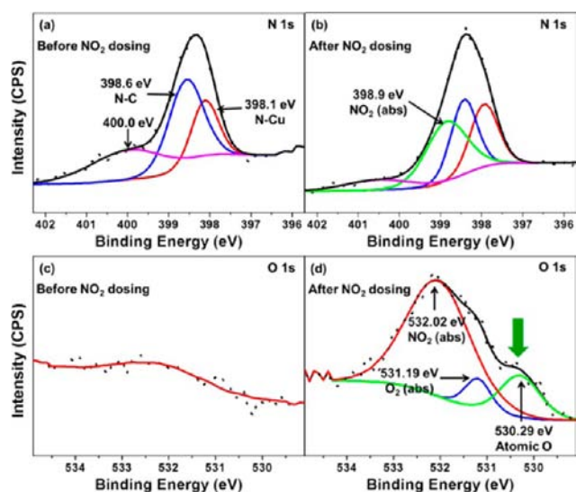
Figure 6. XPS chemical fitting analysis of NO 2 /CuPc/Au(111). (a) N 1s spectra taken from CuPc/Au(111) exposed to air for 10 min, (b) N 1s spectra taken from the NO 2 /CuPc/Au(111) is dosed with 10 ppm of NO 2 for 5 min and subsequently annealed at 50 °C for 20 min. (c) O 1s spectra taken from CuPc/Au(111) exposed to air for 10 min, (d) O 1s spectra taken from the NO 2 /CuPc/Au(111) dosed with 10 ppm of NO 2 for 5 min and subsequently annealed at 50 °C for 20 min.
