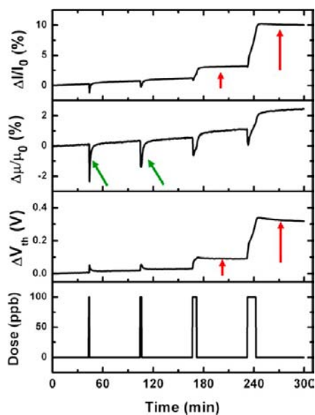
Figure 1. Conductive sensing response of CuPc OTFTs to 100 ppb of NO 2 gas pulses of variable duration. The pulses were 30 s, 2 min, 5 min, and 10 min, resulting in integrated doses of 0.05–1 ppm min -1 . Full I–V characterization was performed at each time point to extract the threshold voltage and mobility. For low doses there is a reversible change in mobility (green arrow), while for high doses there is an irreversible shift in threshold voltage (red arrow).
